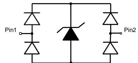
Pin configuration
