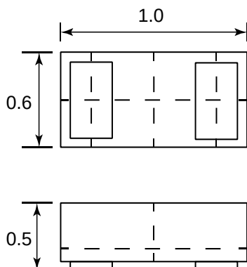
Package Dimensions
