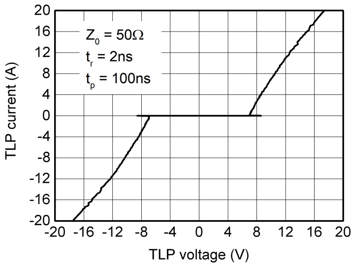
TLP Measurement
