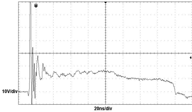
ESD clamping
