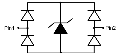
Pin configuration
