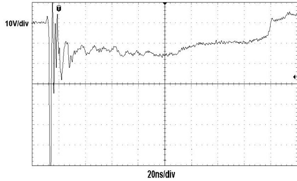
ESD clamping
