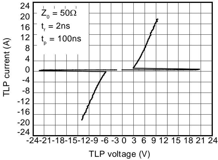
TLP Measurement
