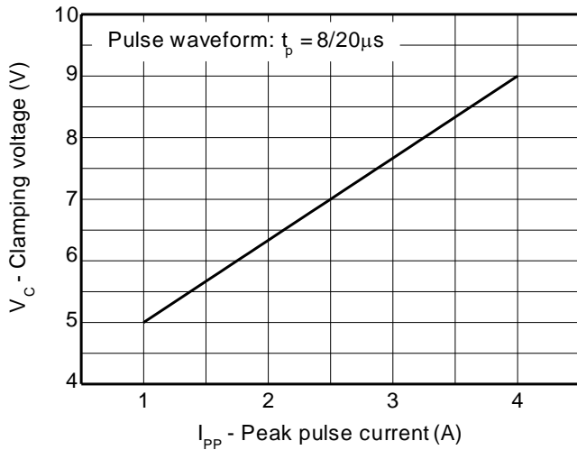
8/20μs waveform per IEC61000-4-5
