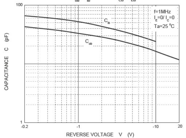
C_{ob}/C_{ib} - V_{CB}/V_{EB}
