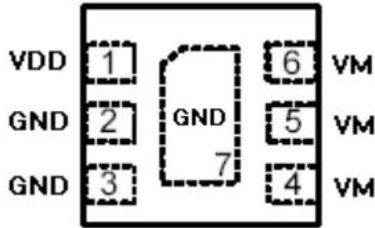
DFN2x2-6
