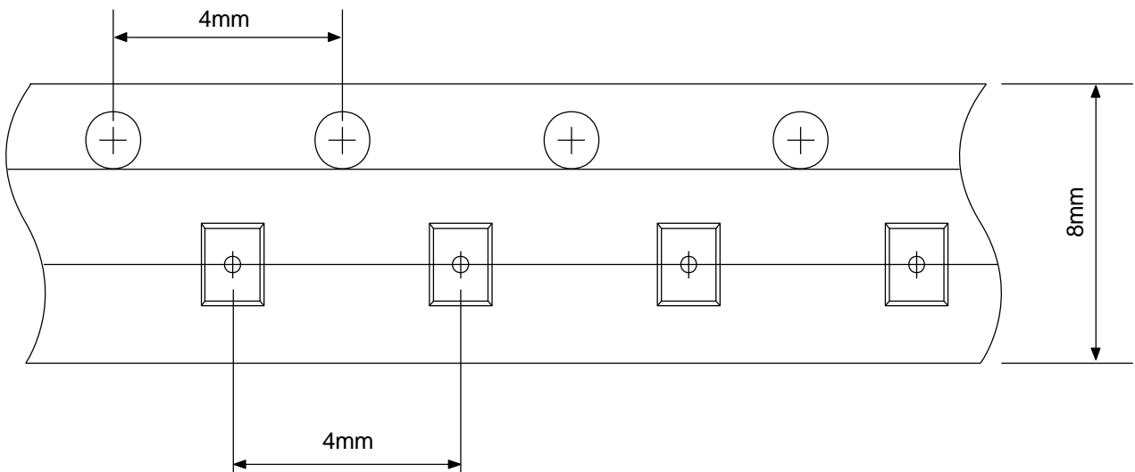
Tape Dimensions
